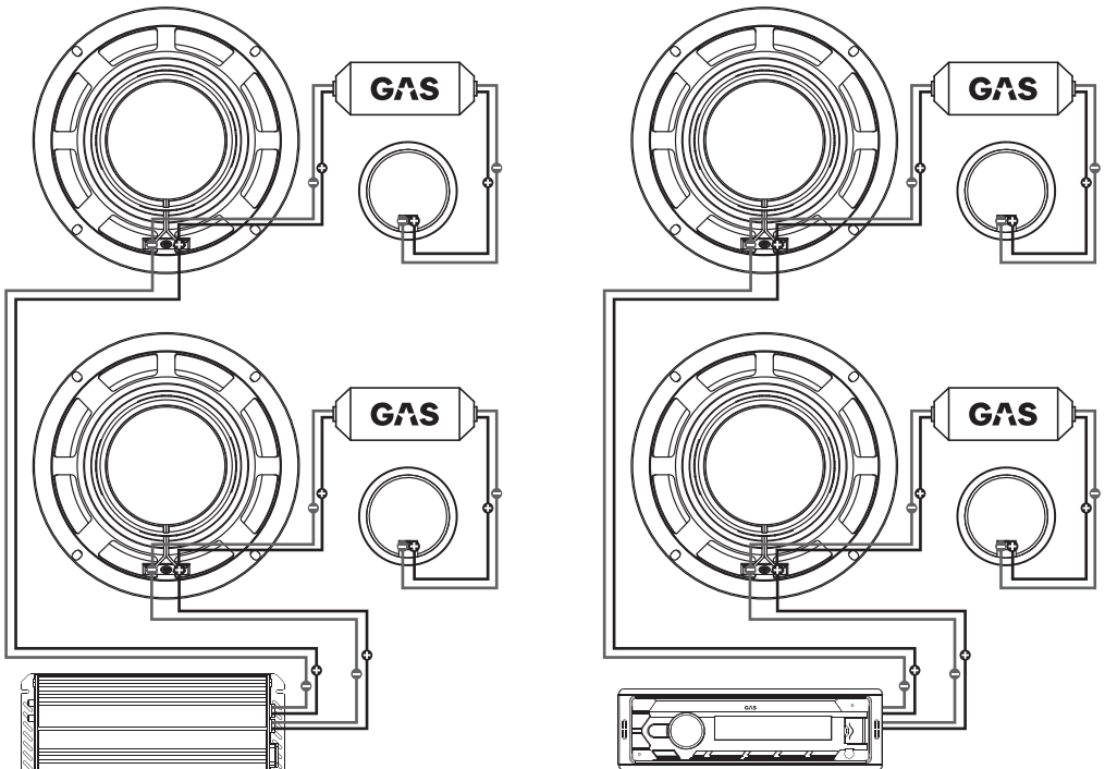
Two 4 Ohm speakers connected directly to a stereo @ 4 Ohm
