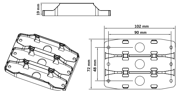
Part No. 850449 TRIPLE MOUNTING BRACKET
