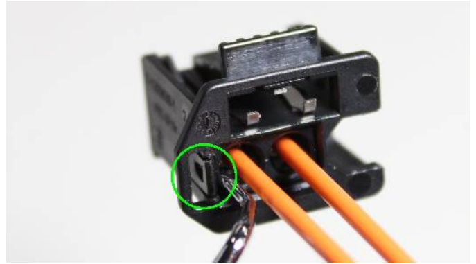
2. Use pick to release tab to take out supplied fiber-optic sub connector (circled in Green)
