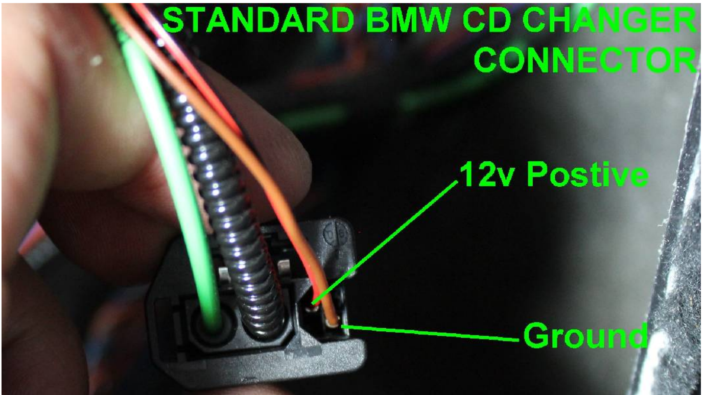
Image A. Standard BMW CD Changer Connector
