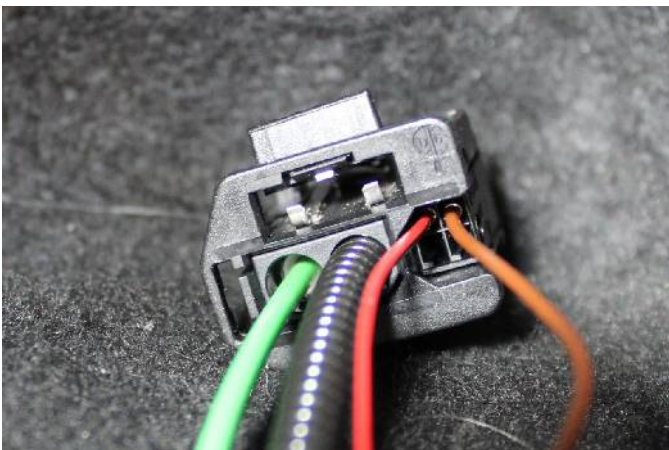
1. Factory fiber-optic Connector showing original Ground wire placement
